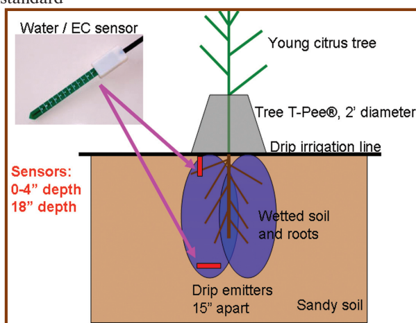
Figure 1. Tested configuration for planting Florida citrus in an ACPS (The tree guard is optional).
